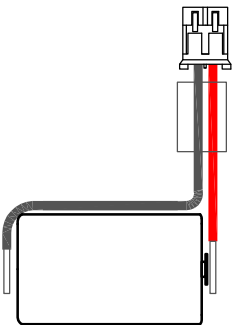
JST-PHR-2P connector
